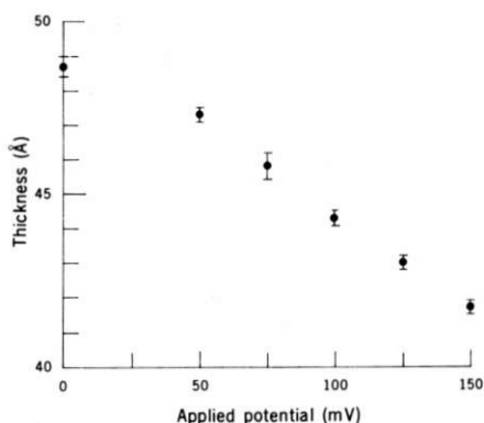
Fig. 1. Thickness of black lipid bilayer membranes as a function of applied potential. The bilayers were formed at 20°C from GMO and n -decane (10 mg/ml) in 0.1M NaCl solutions. Thickness ( \delta_B ) is calculated from measurements of specific geometric capacitance C_g (Table 1) as described in (19).
