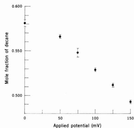
Fig. 2. Apparent mole fraction of n -decane in GMO/ n -decane bilayers as a function of applied potential. Mole fraction ( X_A^b ) is calculated from measurements of specific geometric capacitance C_g (Table 1) as described in (19).
